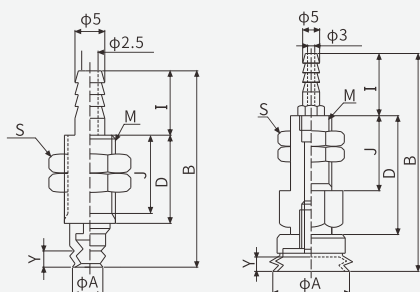
Vertical direction connection - Pagoda fitting
